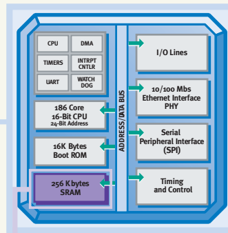
EX Chip Hardware Diagram
